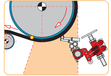
CT – Operating Position The CT can be positioned in the area shown above, on the head pulley.
