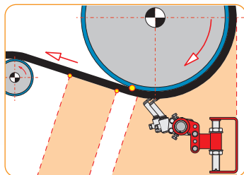
C1 – Operating Position Universal scraper that can be installed either on the head pulley or in the under belt position.
